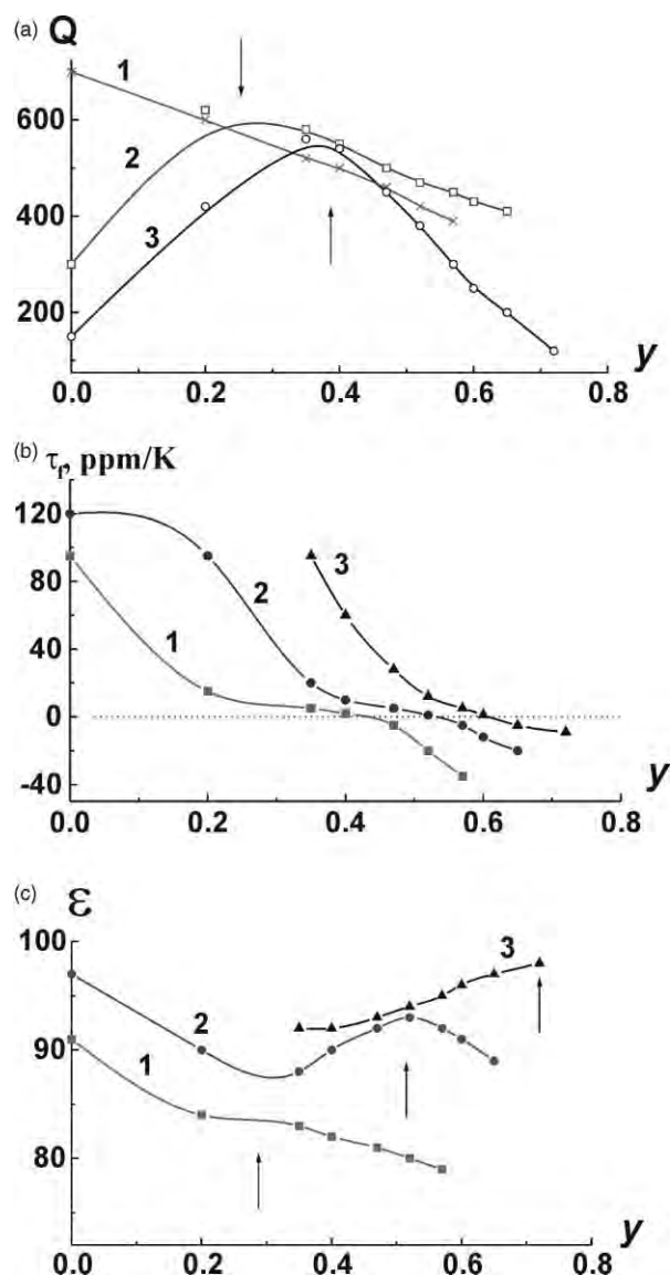
Fig. 4. Dielectric characteristics: (a) Q -value; (b) temperature coefficient of resonant frequency ( \tau_f ); (c) dielectric constant ( \epsilon ) of the (\text{Ba}_{1-y}\text{Pb}_y)_{6-x}\text{Nd}_{8+2x/3}\text{Ti}_{18}\text{O}_{54} system as a function of Pb concentration, measured at 10 GHz. (1) x=1.5 ; (2) x=0.75 ; (3) x=0 .
